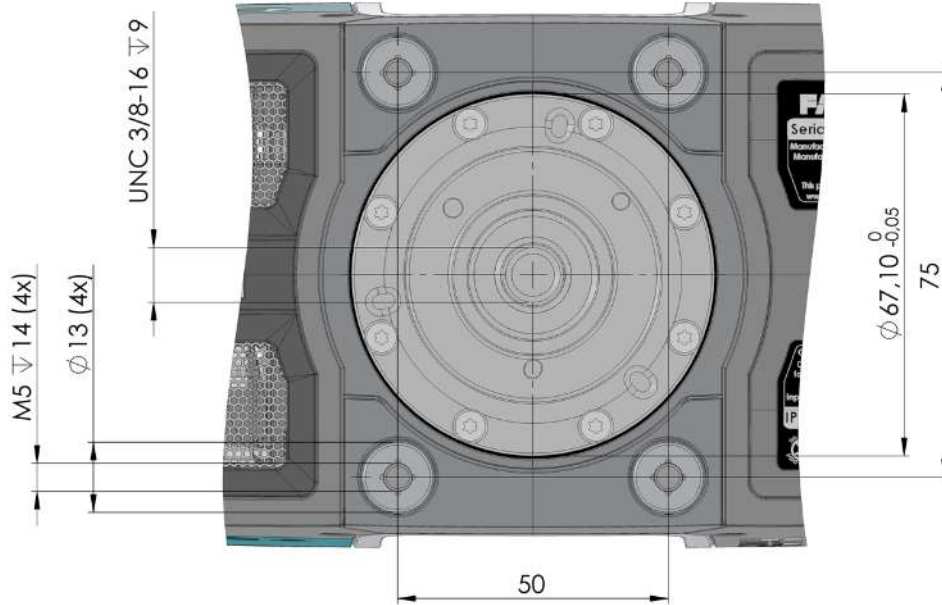
Figure 9-2 Scanner mount
