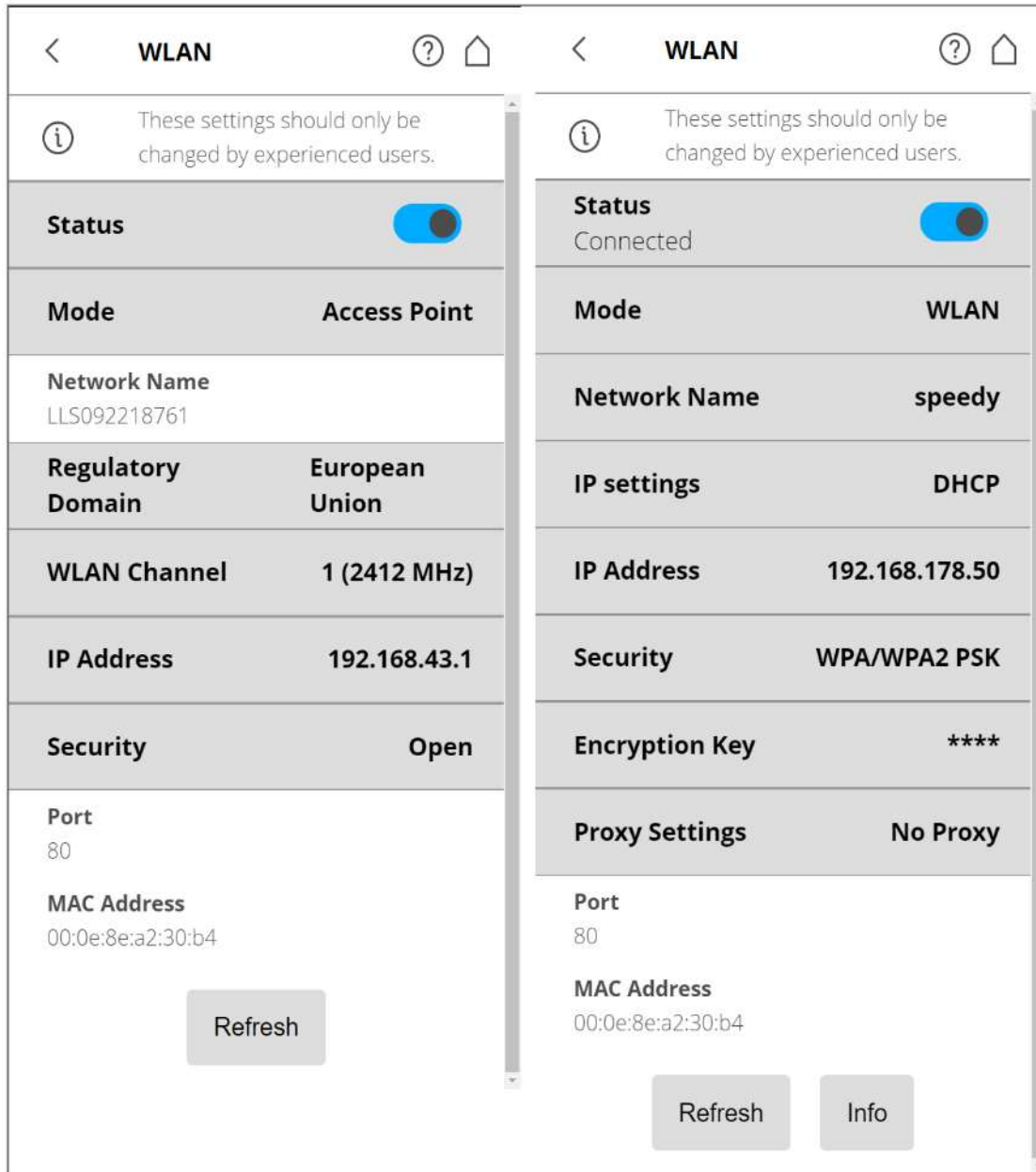
Figure 6-21 WLAN Settings
