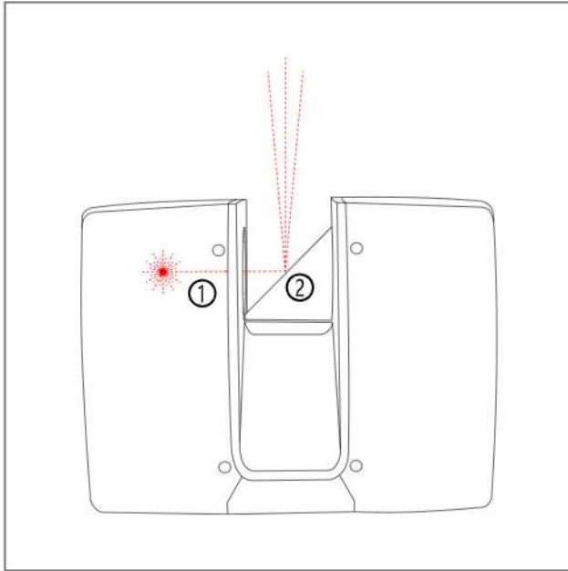
Figure 2-2 Laser Deflection
