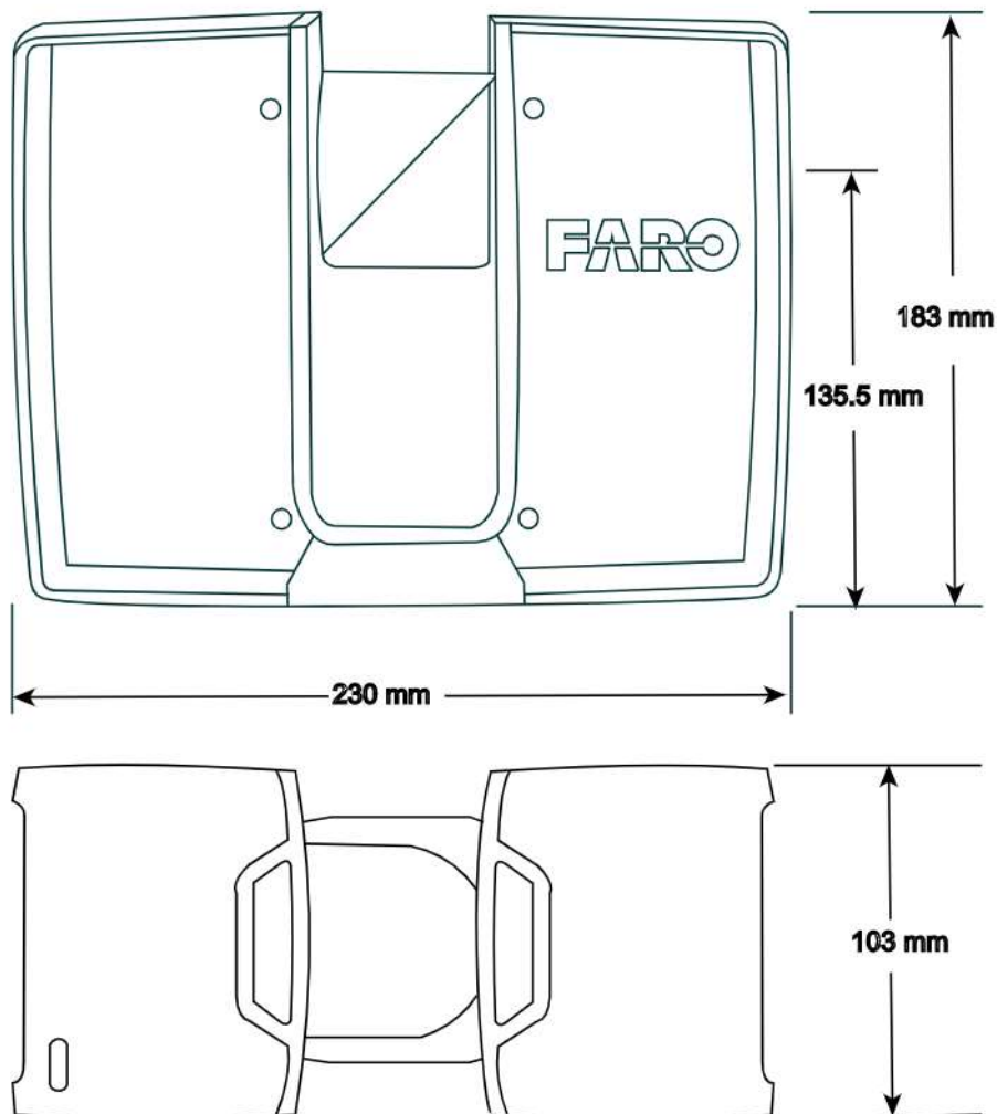
Figure 9-1 Scanner Dimensions
